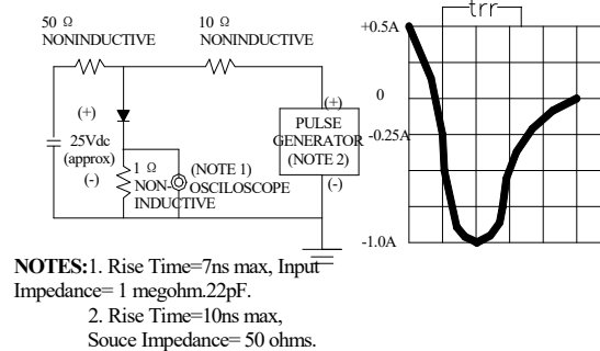
FIG.6-TEST CIRCUIT DIAGRAM AND REVERSE RECOVERY TIME CHARACTERISTIC
